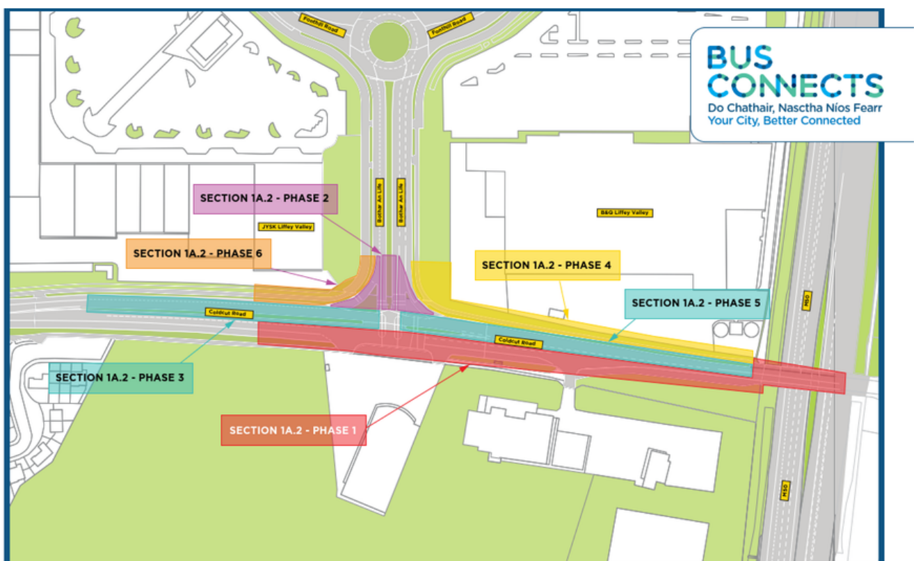
Figure 1: Works area and construction phases (Phases 1–6)
