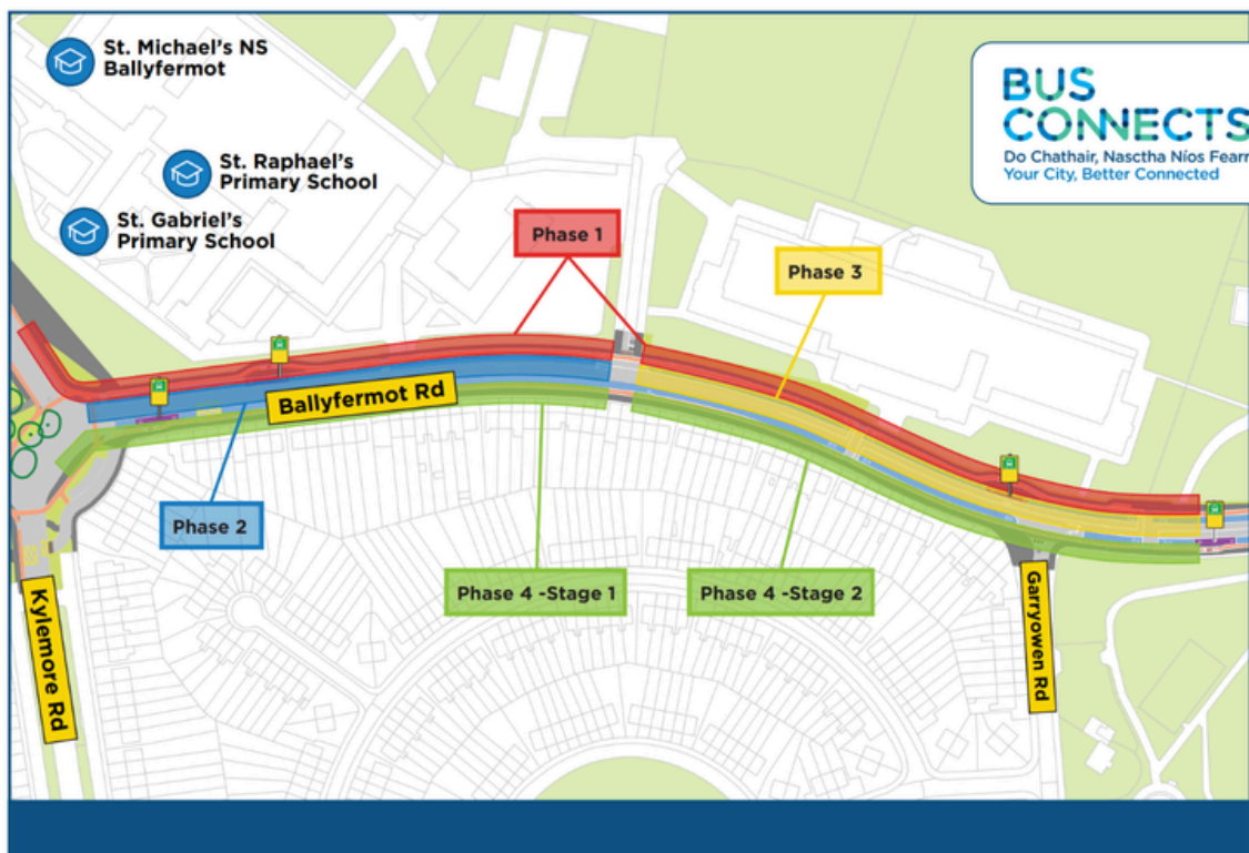
Figure 1: Works area and construction phases (Phases 1-4)
